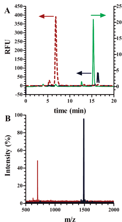
Figure 3. Chromatograms (A) and mass spectra (B) of the fragments formed upon cleavage of MMP-RGD by purified active MMP-2. Elution of uncleaved MMP-RGD (blue —, 16.4 min) was monitored using \lambda_{Ex} 490 nm/ \lambda_{Em} 570 nm. Elution of VRGK(TAMRA)-Aeea-GRGDS (red —, 6.9 min) and FAM-GPLG (green —, 15.4 min) fragments was monitored using \lambda_{Ex} 540 nm/ \lambda_{Em} 570 nm and \lambda_{Ex} 490 nm/ \lambda_{Em} 535 nm, respectively. Fragments were confirmed to be FAM-GPLG (red —; MW = 701) and VRGK(TAMRA)-Aeea-GRGDS (black —; MW = 1485) by mass spectroscopy. (Data are representative of three independent experiments.)
